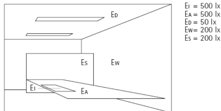
Fig.: Examples for brightness on various locations in a typical office (desk EA = 500 lx)
